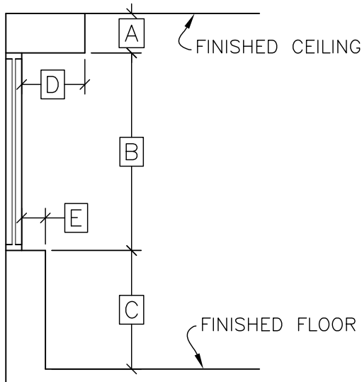
CROSS-SECTION OF EXTERIOR WINDOW CONDITION
